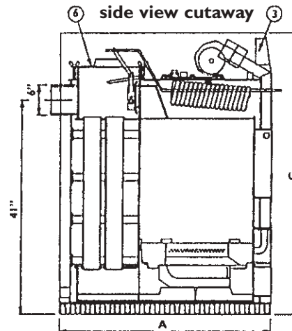
Solo Plus 30-40 side view cutaway
