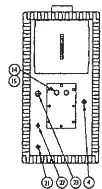
Solo Plus 30-40 seen from above
