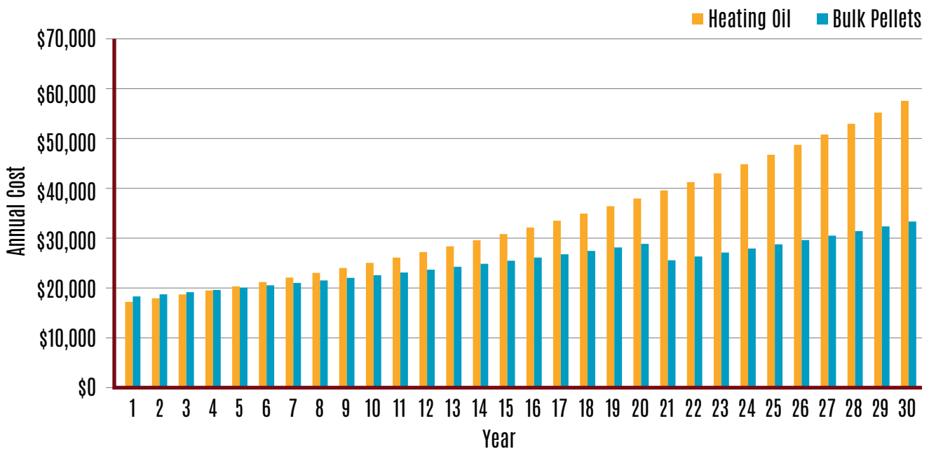
FIGURE 16: Example of a 30-year economic analysis comparing the annual costs of heating oil vs. a new wood heating system
